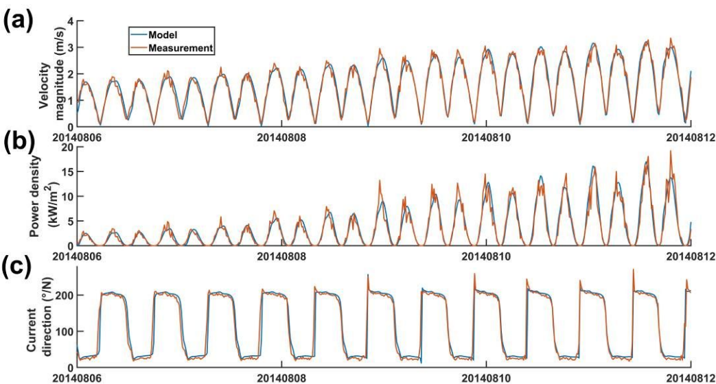
Figure 2: Time-series of horizontal current magnitude (a), power density (b) and current direction at hub height (c). The blue curve represents model predictions. The red curve represents measurements by ADCP. The time-series were extracted 15 m above the seabed. Reprinted from [20] Thiébot et al. (2020) Wake field study of tidal turbines under realistic flow conditions. Renewable Energy, https://doi.org/10.1016/j.renene.2019.11.129 . Copyright 2020, with permission from Elsevier.
