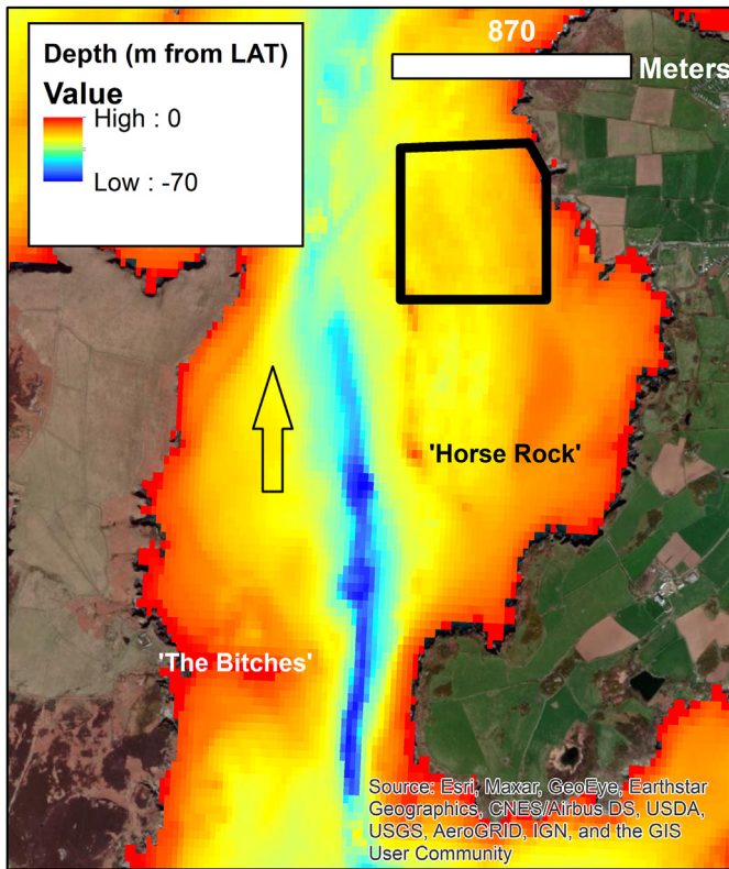
Fig. 2. The Bathymetry of Ramsey Sound with key features labels and the flight area indicated as a black polygon. The black outline arrow indicates direction of the flood tide. Bathymetry [79] © British Crown and OceanWise, 2021. All rights reserved. Licence No. EK001-20180802. Not to be used for Navigation.
