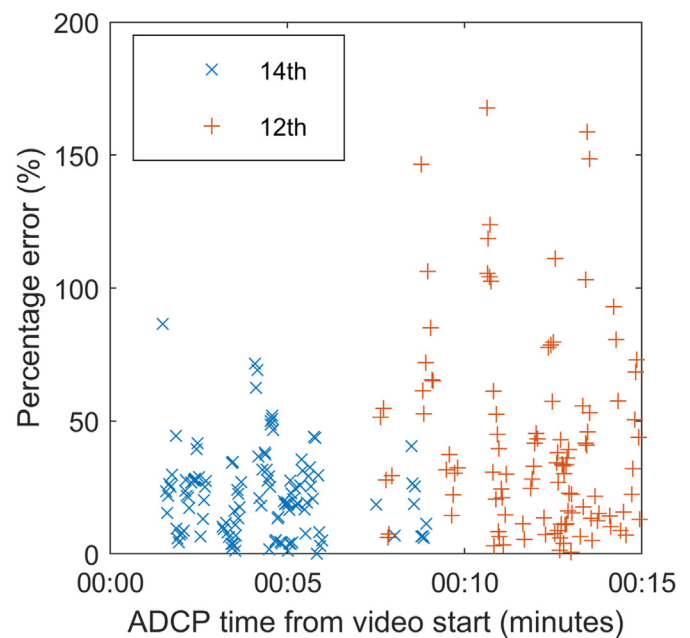
Fig. 15. A comparison between error and temporal separation of ADCP recording to video start time from the Ramsey Sound survey location. Dates correspond to the two survey dates in May 2021.
