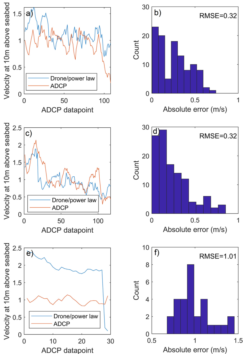
Fig. 19. A comparison between ADCP velocities measured at 10m above the seabed and velocities at 10m above seabed estimated from drone measured surface velocities and the power law profile. Comparative plots of the two velocities are given for a) Ramsey Sound on the 12th May, c) Ramsey Sound on the 14th May, e) Inner Sound. Error histograms are given for b) Ramsey Sound on the 12th May, d) Ramsey Sound on the 14th May, f) Inner Sound.
