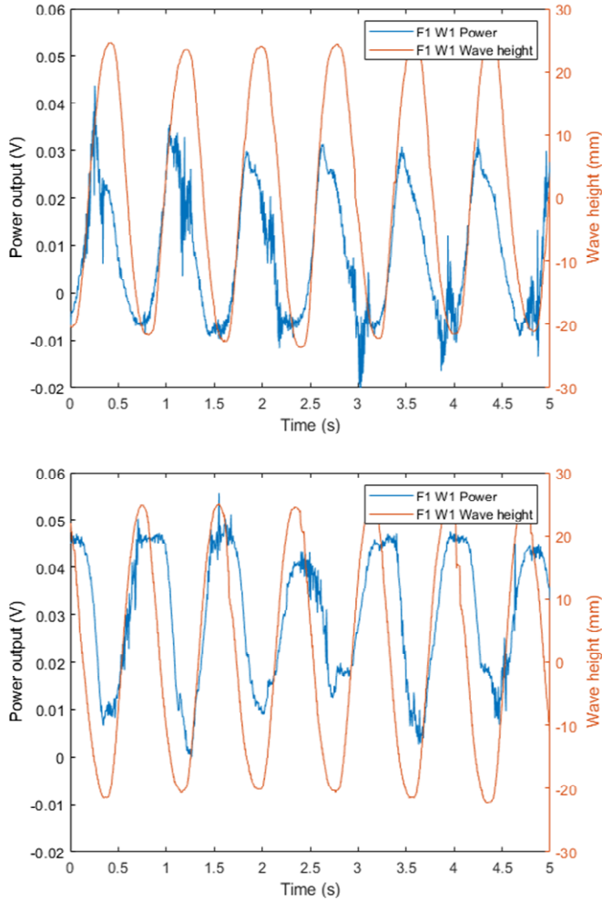
Figure 6: Power generation data for flow case 1 (1.3 m/s) with wave case 1 (4.0 m waves at 7.2 s period) for turbine mounted on a fixed (top) and floating (bottom) support structure
