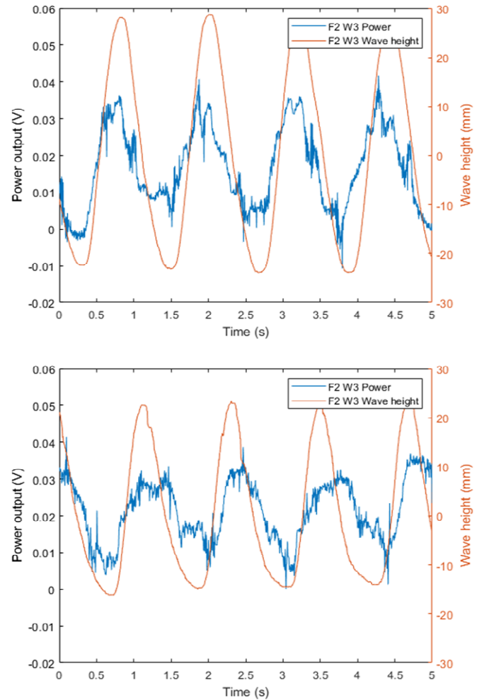
Figure 7: Power generation data for flow case 2 (1.7 m/s) with wave case 3 (4.0 m waves at 10.8 s period) for turbine mounted on a fixed (top) and floating (bottom) support structure.
