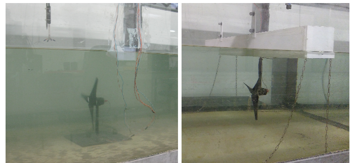
Figure 5: Turbine mounted on fixed (l) and floating (r) support structures
