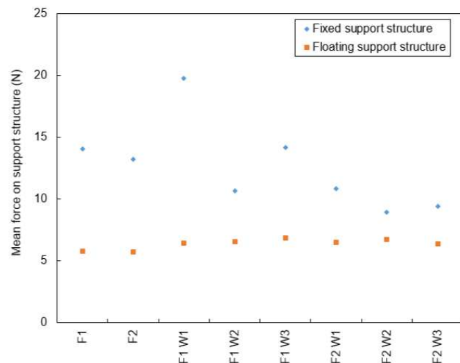
Figure 9: Mean support structure force experienced by fixed and floating support structures in all flow and wave cases (as per Table 1).
