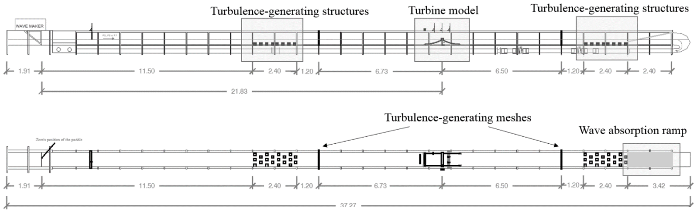
Figure 3: Wave-Current flume layout and turbine model position during tests at LABIMA.
