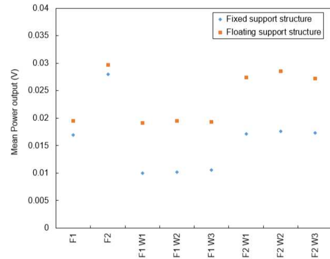
Figure 8: Mean power generation for turbine mounted on fixed and floating support structure in all flow and wave cases (as Table 1). Mean power generation for 10,000 samples during wave generation period (excl. F1 and F2 cases).
