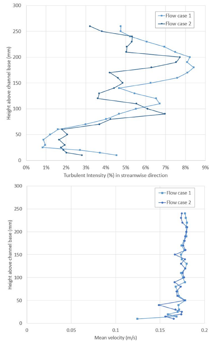
Figure 4: Turbulent intensity (top) and mean streamwise flow velocity (bottom) recorded in the LABIMA Wave-Current flume for flow cases 1 and 2.
