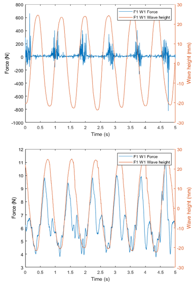
Figure 10: Support structure force flow case 1 (1.3 m/s) with wave case 1 (4.0 m waves at 7.2 s period) for turbine mounted on a fixed (top) and floating (bottom) support structure.
