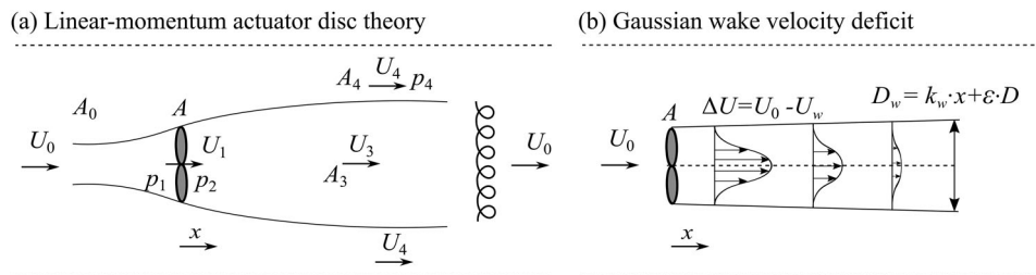
Figure 1 Theoretical representation of the wake behind a single tidal turbine adopting (a) linear-momentum actuator disc theory where U denotes streamwise velocity, A area and p pressure with a subscript denoting location (adapted from Garrett & Cummins, 2013); and (b) Gaussian wake velocity field in which \Delta U denotes velocity deficit, x distance downstream of the rotor, D rotor diameter and the wake width is represented by D_w with k_w the wake expansion rate and \varepsilon \cdot D the onset wake width
