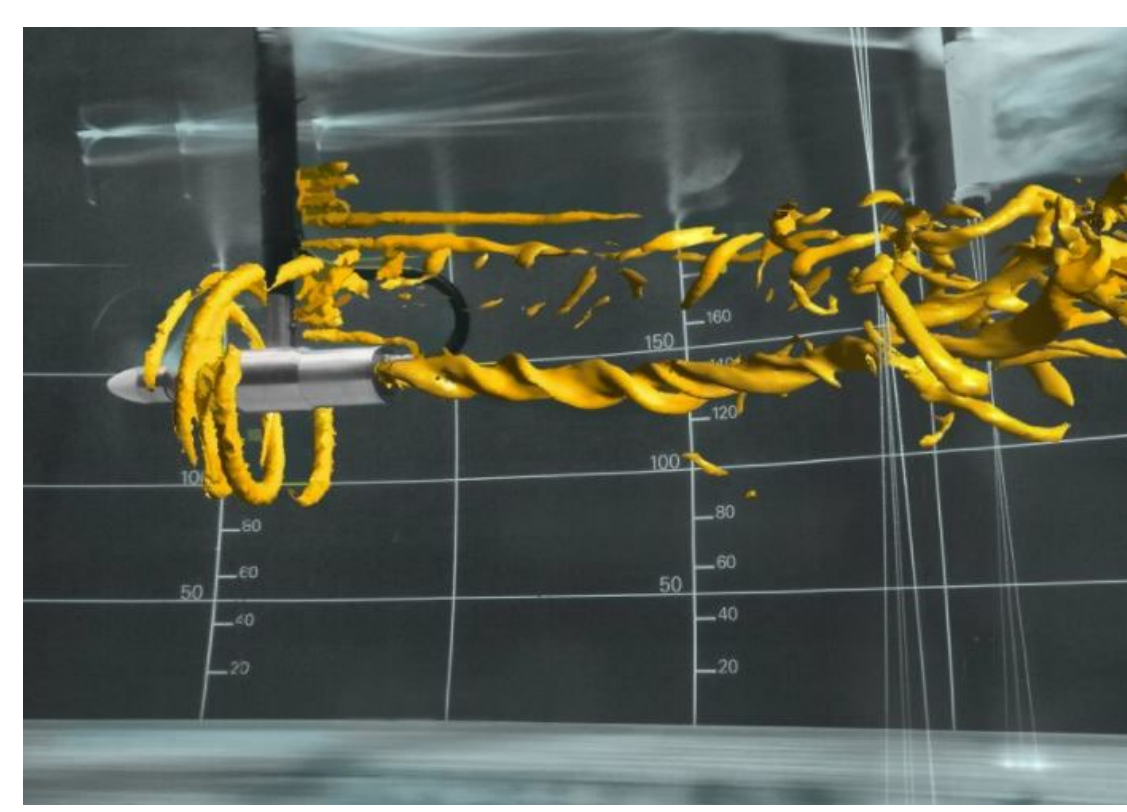
Figure 2: Turbulence in TST © CMERG
