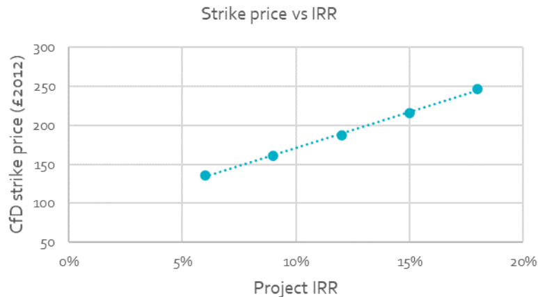
Figure 11 – CfD strike price vs project IRR for the Raz Blanchard Phase 2 baseline scenario.
