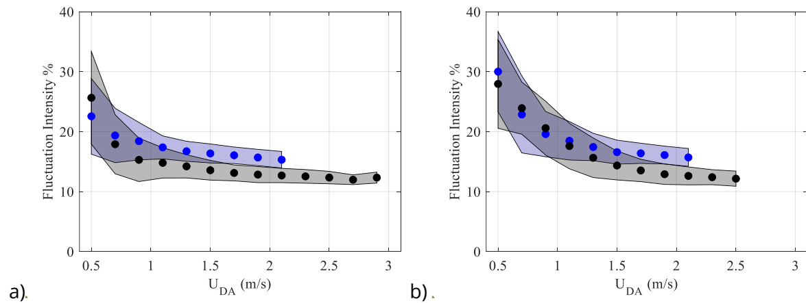
Figure A3. Fluctuation intensity of velocity at two ADCP locations (a and b), for a near-bed turbine for the flood tide (RHS) and the ebb tide (LHS) within the EMEC test site, for a range of disk averaged velocities.
