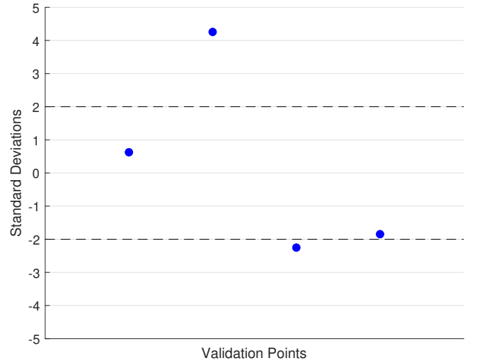
Figure 7. Standard error of predicted values from first iteration of 2D emulator at first four of validation points
